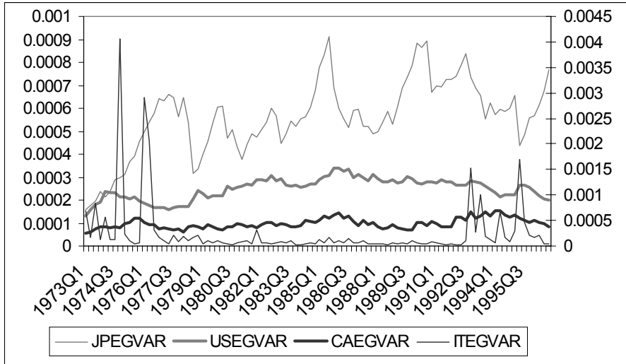
Figure B3. Exponential GARCH conditional volatility
