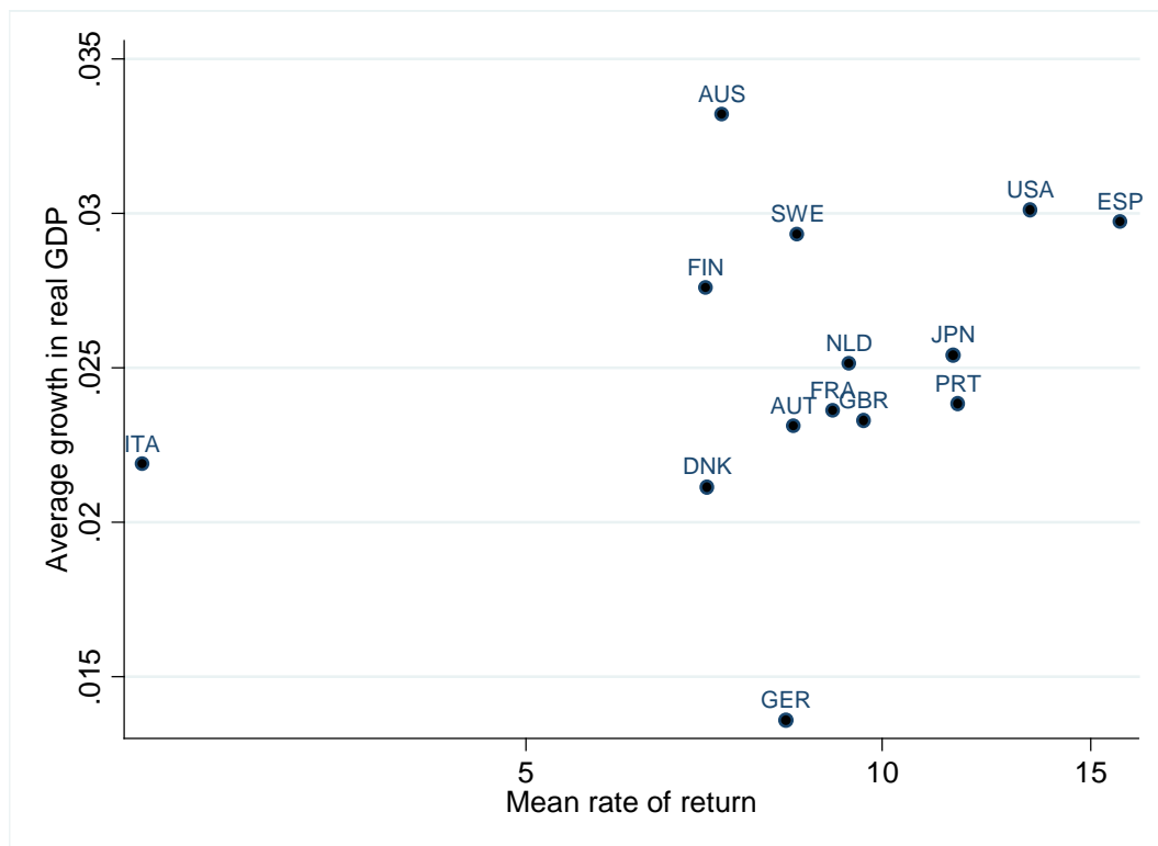
Mean growth rate of real GDP versus mean real rate of return in the market economy
